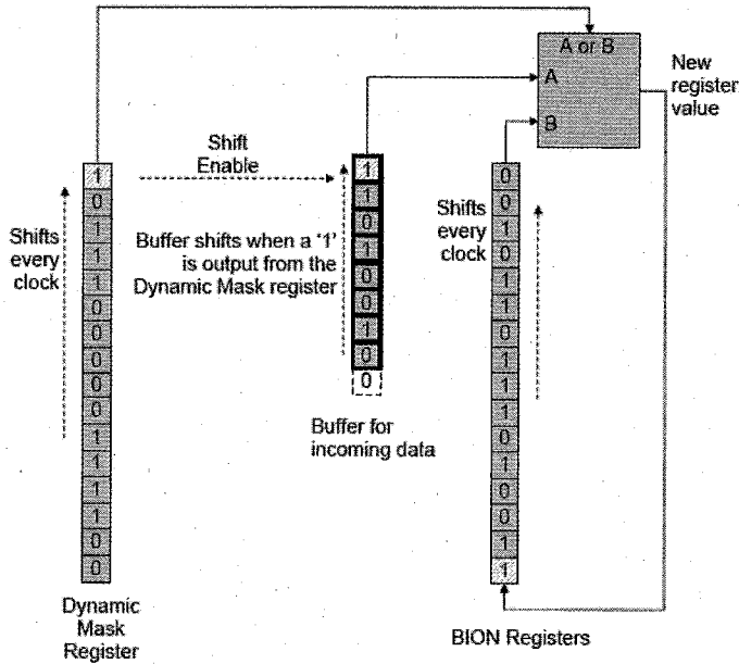
Fig. 4. Dynamic mask operation.
