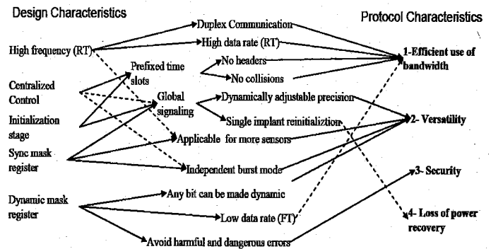
Fig. 8. Summary of protocol characteristics.
